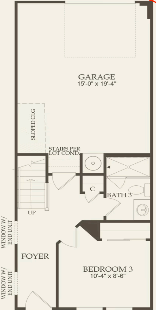
First Floor w/ Bedroom/Bath I.L.O Tandem Garage
