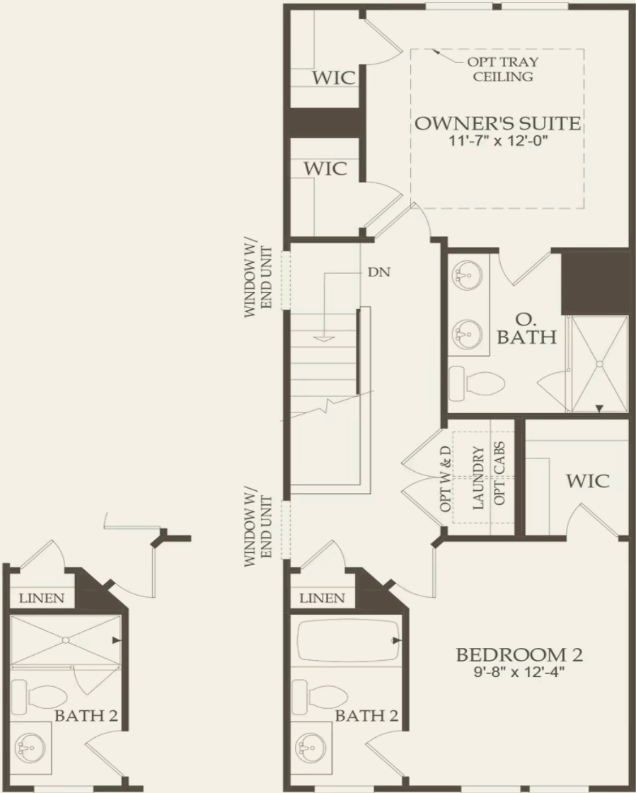
Opt. Shower at Bath 2
